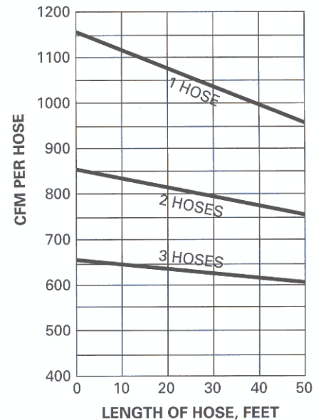
F66 WITH SOURCE CAPTURE PLENUM AND 8" HOSE
